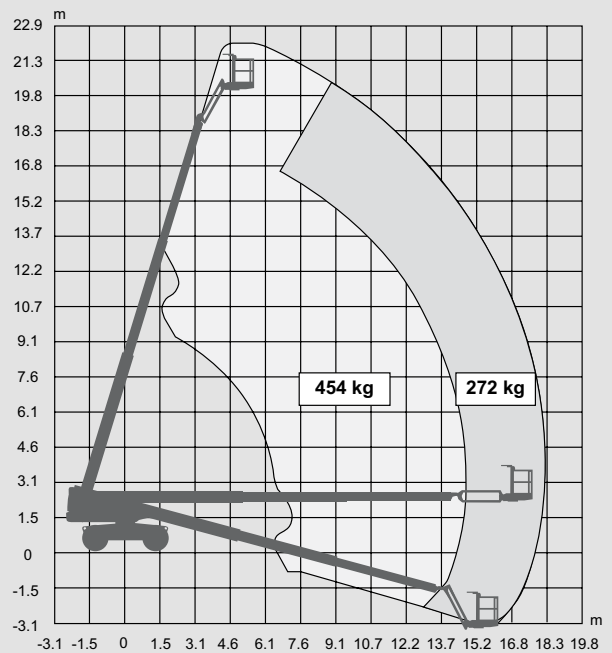
SJ66 T+ WORKING ENVELOPE
